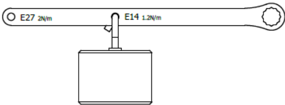
weight position for E14
